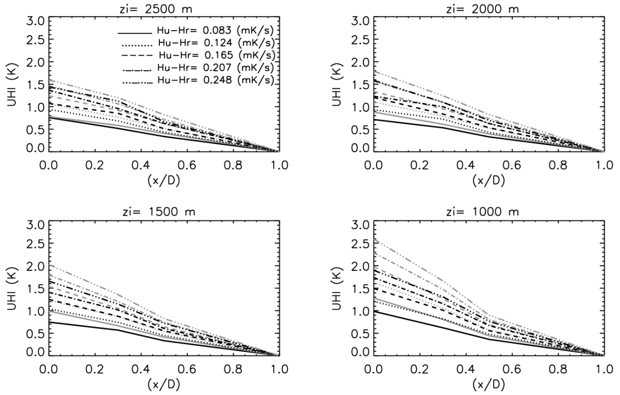
Figure 5: (a) Horizontal profiles of surface temperature distribution as a function of the nondimensional distance (x/D) . The black line corresponds to the D = 10 km and the grey line to the D = 20 km simulations, respectively.
