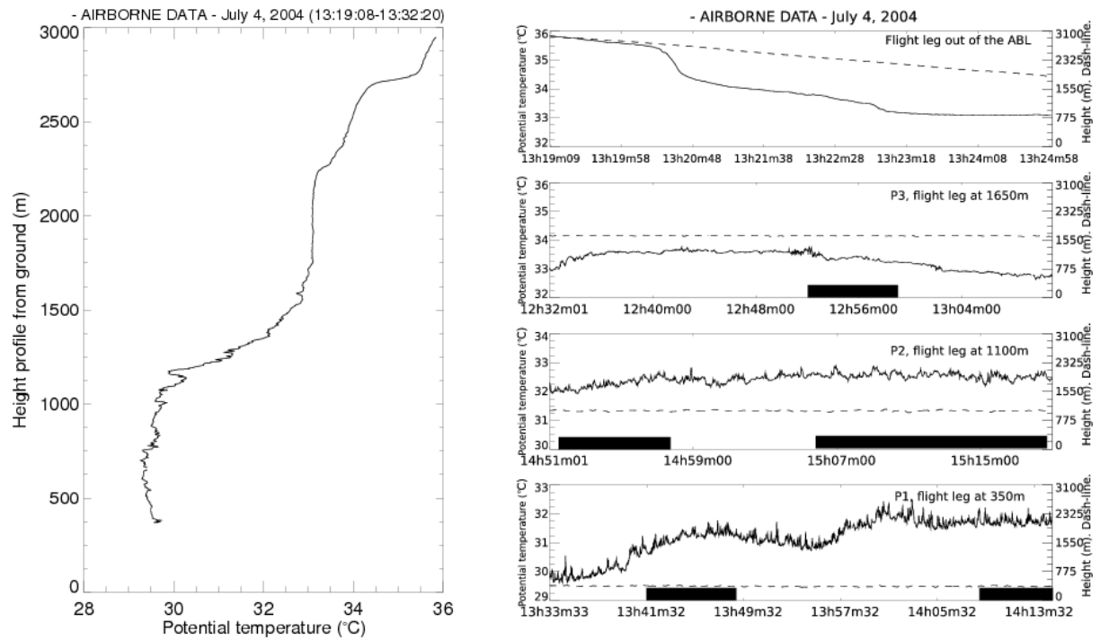
Figure 6 a and b: Vertical profile of potential temperature from the airborne sounding in the rural zone at 13.20 UTC (a). Temporal evolution of potential temperature observed by the aircraft (b) at height of 350 m, 1100 m and 1650 m. And a vertical profile of potential temperature from 3000 m to 1950 m. The black strip indicates when the aircraft over flies Toulouse.
