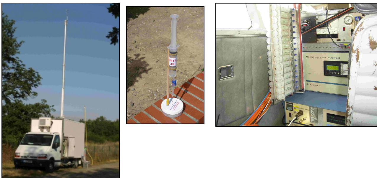
Figure 6: Instruments to measure \text{SF}_6 dispersion: a: The laboratory van equipped with a telescopic 10 m mast. \text{SF}_6 is released at 2m50 of height (seen behind the van). b: Ground sampling with a drop by drop system. c: Aircraft rack including 30 gas syringes.
