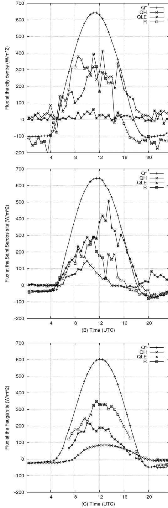
Figure 3 a and b: Energy balance components for the 4 th July 2004 in the central tower (a) and in the rural sites (Saint Sardos, b and Fauga, c). Flux densities of net all-wave radiation ( Q^* ), sensible heat ( Q_H ), latent heat ( Q_{LE} ) and the residual term calculated as R = Q^* - (Q_{LE} + Q_H) .
