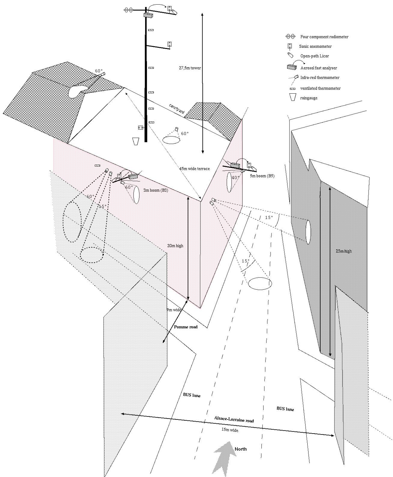
Figure 3: Schematic view of the central site
