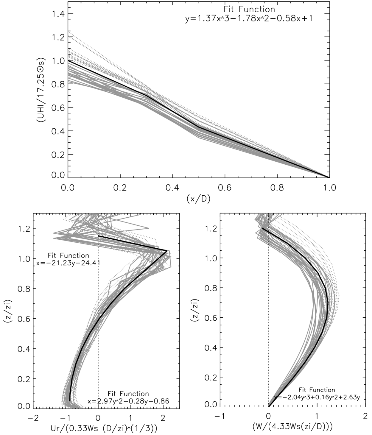
Figure 8a: Normalised horizontal profiles of surface temperature distribution (12 m of height) from the centre of the domain (top), radial velocity (down left) and vertical velocity (down right). The continuous grey line corresponds to the D = 10 km simulation, the dotted grey line to the D = 20 km simulation, and the black lines represent the best least square polynomial fit.
