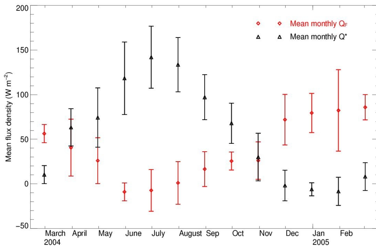
Figure 7: Annual cycle of net radiation (black) measured at the top of the central site tower, and of anthropogenic heat flux (red), estimated from the integrated residual method. Vertical bars indicate day-to-day variability.
