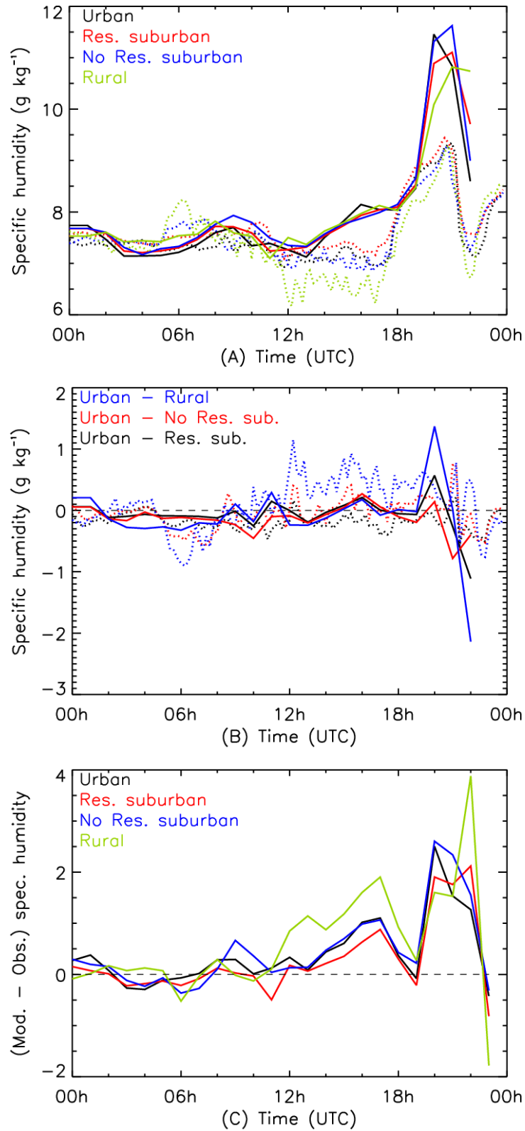
Figure 6: Temporal evolution of observed and modelled 2m air specific humidity (a), humidity island (b) and bias (c), the 4 th July. Output values from the simulation URB and the model M4 at 2 m have been extracted at grid points corresponding to the location of the surface stations and averaged by urbanization class.
