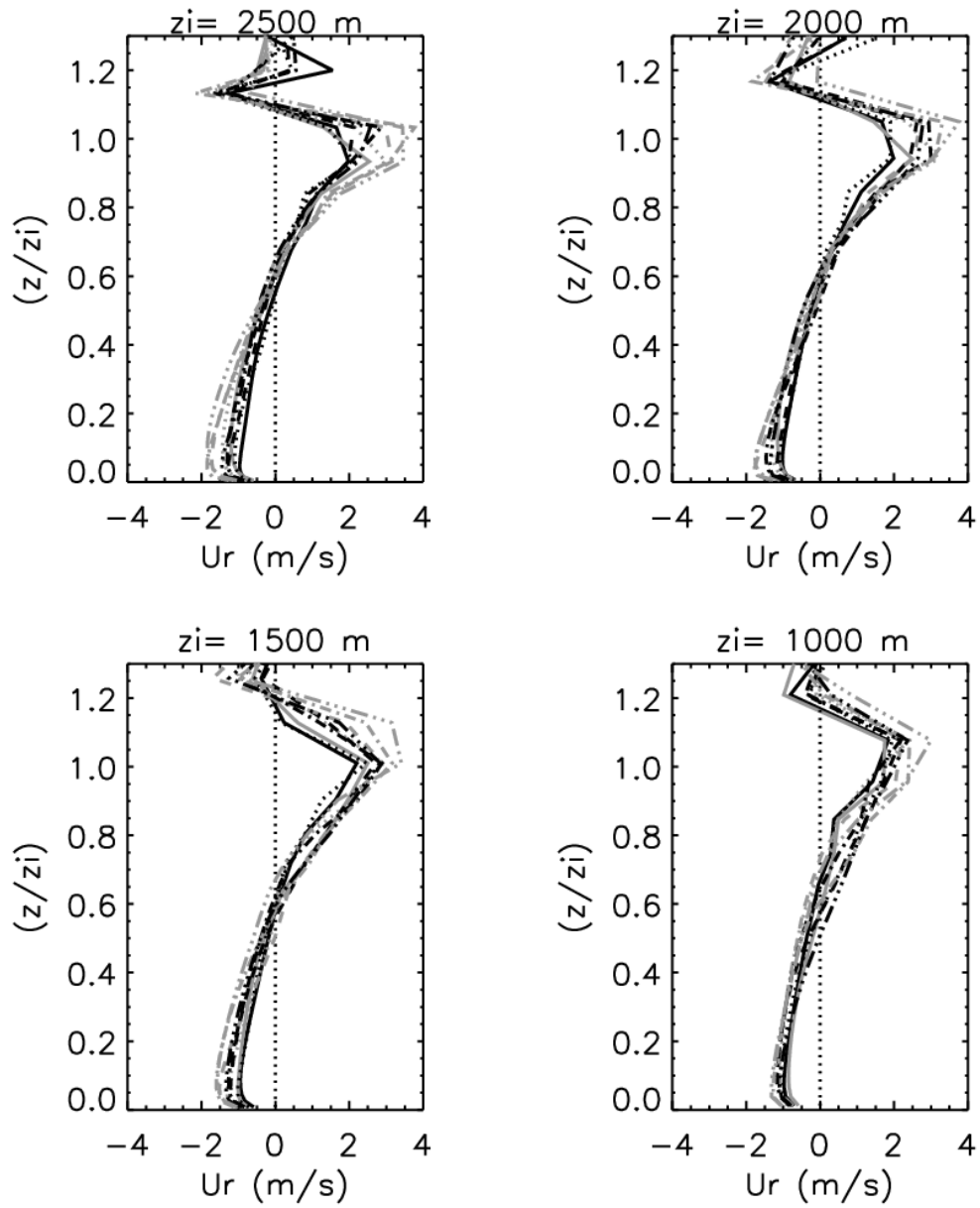
Figure 6: (b) Vertical profiles of radial velocity as a function of the nondimensional height ( z/z_i ) for the different simulations. The black line corresponds to the D = 10 km and the grey line to the D = 20 km simulations, respectively.
