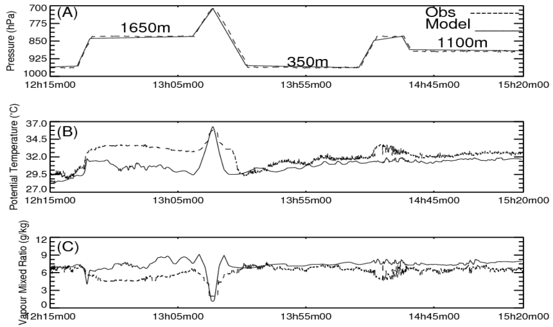
Figure 3: Time series of pressure (a), potential temperature (b) and vapour mixed ratio (c) observed by the Piper Aztec aircraft the 4 July and modelled by MesoNH (URB(M4) and URB(M3) when the aircraft goes out of the M4 domain).
