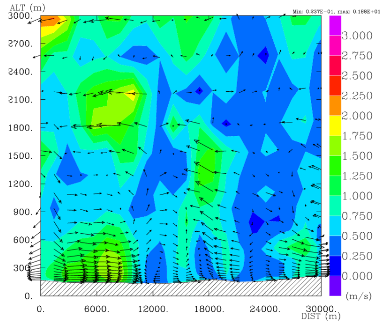
Figure 8: Vertical NW-SE cross-section of the anomaly wind ( M3_{URB}-M3_{RUR} ) between 12.30 to 15.30 UTC (a) and to 15.00 to 18.00 UTC (b) over plotted to the horizontal wind intensity. The horizontal projection of the vertical cross-section is in Figure 7b.
