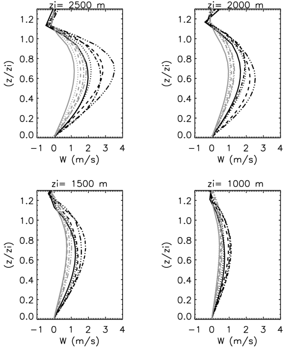
Figure 7: (c) Vertical profiles of vertical velocity as a function of the nondimensional height ( z/z_i ) for the different simulations. The black line corresponds to the D = 10 km and the grey line to the D = 20 km simulations, respectively.
